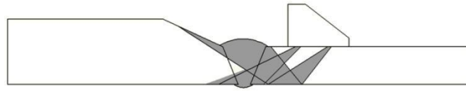
Figure A1.2(b) PAUT Testing From the Scarfing Surface
