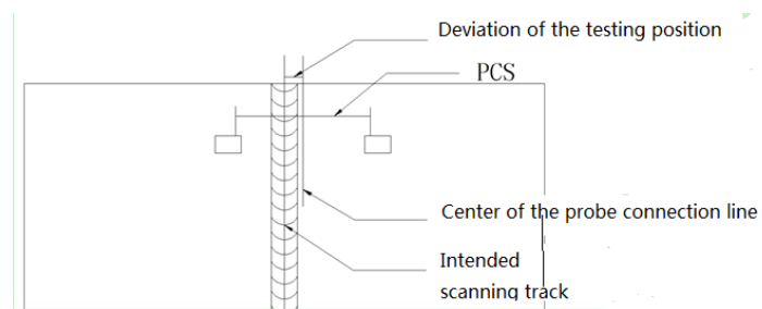
Figure 4.5.1.1 Illustration of TOFD Scanning Deviation
